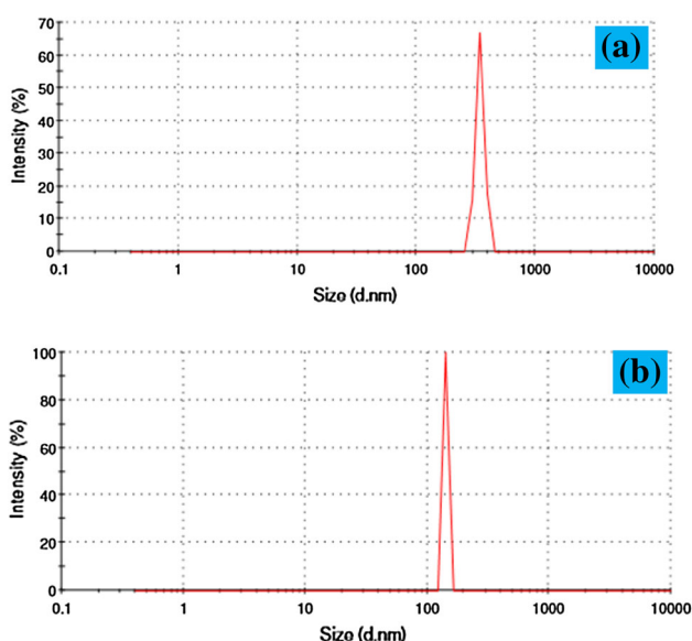
Fig. 7 DLS spectra of (a) Pure ZnO NPs and (b) Co doped ZnO NPs
